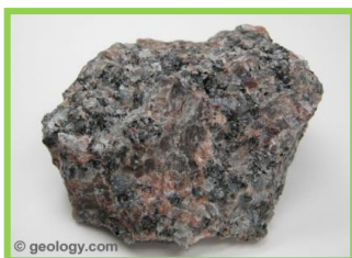
Granite rock
