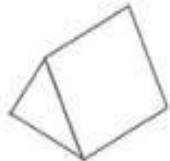
Triangular prism
