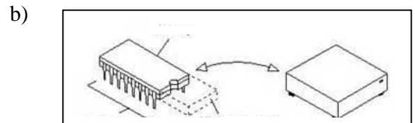
virtual memory
